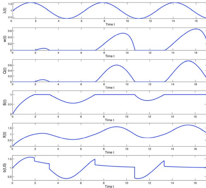
Figure 2. Six performance functions for the G_t / H_2 / s + E_2 fluid model with sinusoidal arrival-rate function \lambda(t) = 1 + 0.6\sin(t) for service capacity s and mean service and patience times equal to 1: (i) arrival rate \lambda(t) ; (ii) head-of-line waiting time w(t) ; (iii) fluid waiting in queue Q(t) ; (iv) fluid in service B(t) ; (v) total fluid in system X(t) ; and (vi) rate into service b(t, 0) .
