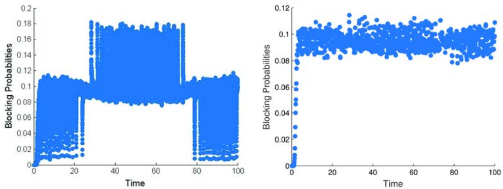
Figure 4. Simulation estimates of the blocking probabilities in the nonstationary M_t / M / s_t / 0 model for the sinusoidal arrival rate in (4.19) with blocking probability target B = 0.1 and parameter triple (\bar{\lambda}, \beta, T) = (100, 25, 100) with the MOL staffing algorithm without any averaging (left) and with randomization (right).
