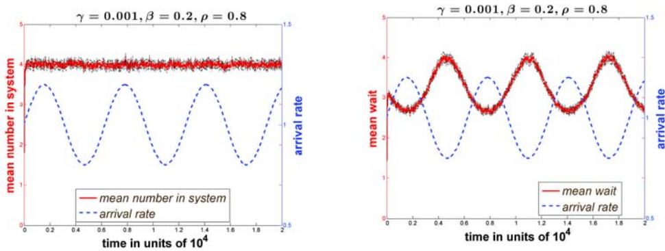
Figure 8. Simulation estimates of the time-varying mean number in the system (left) and the mean virtual waiting time (right), for the M_t / M_t / 1 model with sinusoidal arrival rate function \lambda(t) = 1 + \beta \sin \gamma t with \beta = 0.2 and \gamma = 0.001 with the rate-matching control in (7.51) for traffic intensity \rho = 0.8 .
