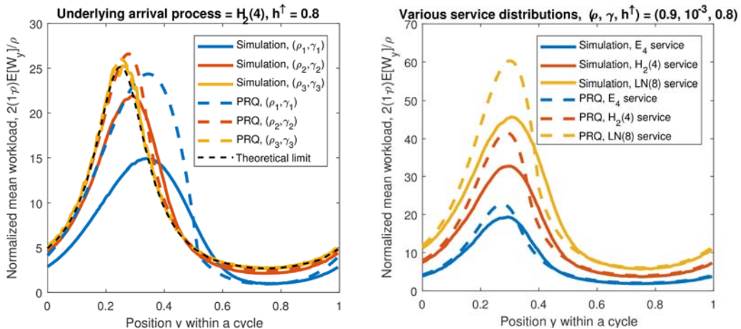
Figure 7. A comparison of the solution to the PRQ problem in (7.43) as a function of the position y within a cycle to simulation estimations and the HT limit in Theorem 5 of Whitt and You [227] for the normalized mean workload 2(1 - \rho)E[W_{\gamma,\rho,y}]/\rho for W_{\gamma,\rho,y} in (7.42) in the underloaded ( H_2(4)_t / LN(1) / 1 ) model with arrival-rate function in (7.47) for (\gamma, \rho) \in \{(0.7, 10^{-2}), (0.9, 10^{-3}), (0.95, 10^{-4})\} (left) and for three different service-time distributions (right).
