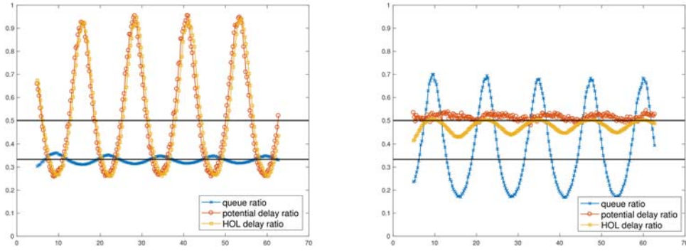
Figure 6. Queue and delay ratios obtained from the FQR rule (left) and HLDR rule (right) for a two-class M_i/M/s_i queue with arrival rate functions \lambda_1(t) = 60 - 20\sin(t/2) , \lambda_2 = 90 + 30\sin(t/2) , common service rate \mu = 1 , without abandonment ( \theta_1 = \theta_2 = 0 ) and the QoS parameter \gamma = 0.25 .
